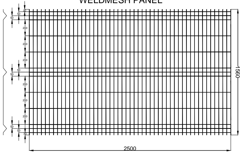
FRONT VIEW - WITH BEND
