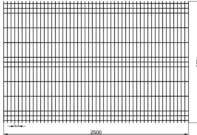
FRONT VIEW - W/O BEND
